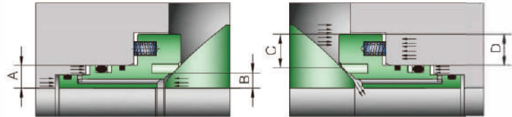
Area (A) > Area (B) Upstream Seat Seal
